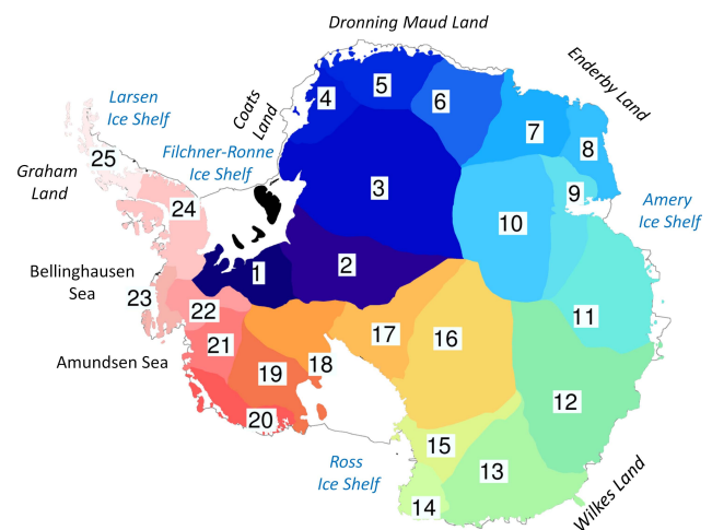
Fig. 1. Division of 25 Antarctic drainage basins investigated in this study (after Rignot et al., 2008; Zwally and Giovinetto, 2011)
